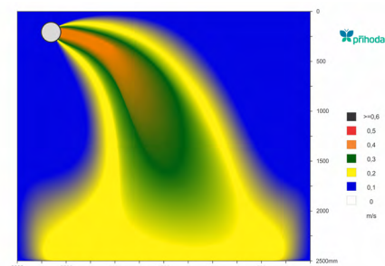
Airflow patterns, microperforation 90^\circ , 165 Pa
