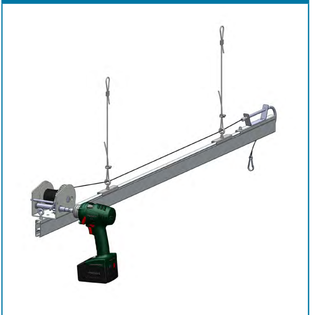
Spoling vha. aku-boremaskine
