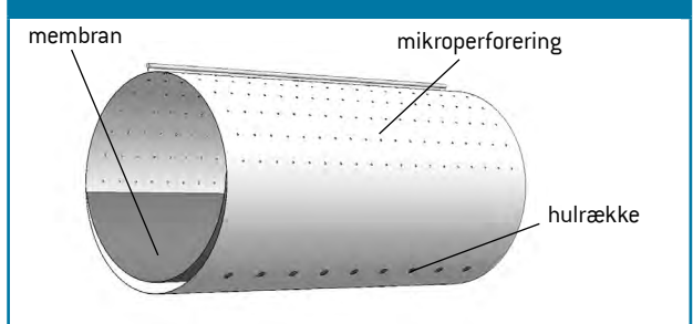
Diffusor
